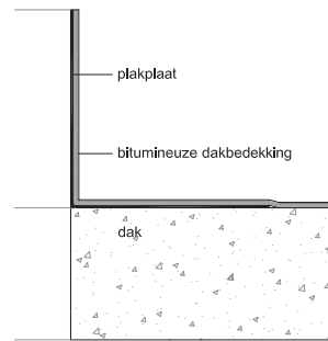
Detail
